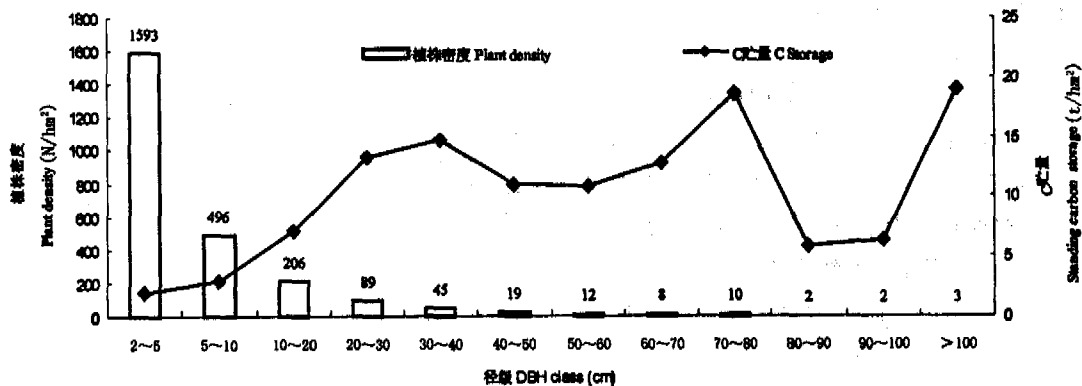
图1 季节雨林乔木层C贮量和植株密度的径级分布状况 Fig. 1 Allocation of standing carbon storage and plant density among the different DBH classes of tree layer
